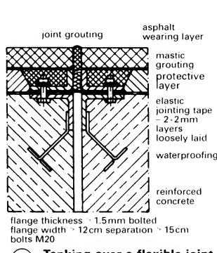
⑧ Tanking over a flexible joint in reinforced concrete slab
